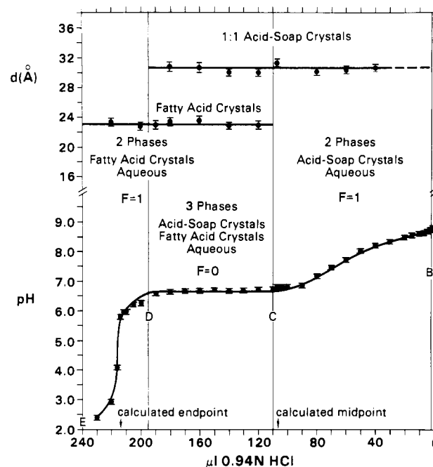
FIGURE 2: Equilibrium titration curve for 0.08 M potassium decanoate with added microliters of 0.94 N HCl at 6 °C. For additional information, see Figure 1 caption.
